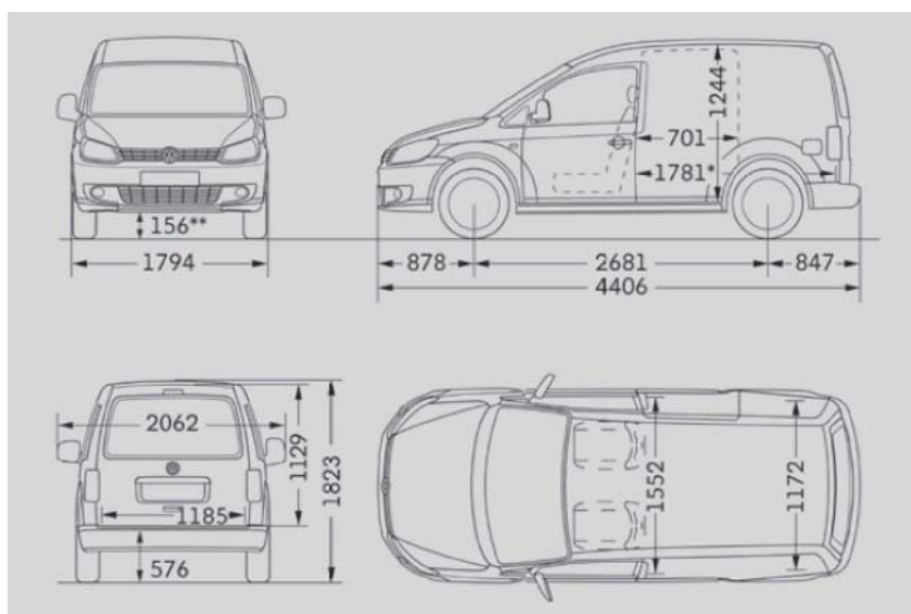
Caddy Van short wheelbase
